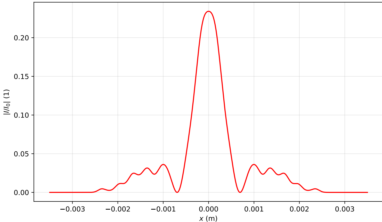
Intensity profile I(x, y = 0, z = 3.582)/I_0 , \text{Pin}=8.0\text{Pcr} , artificial time
